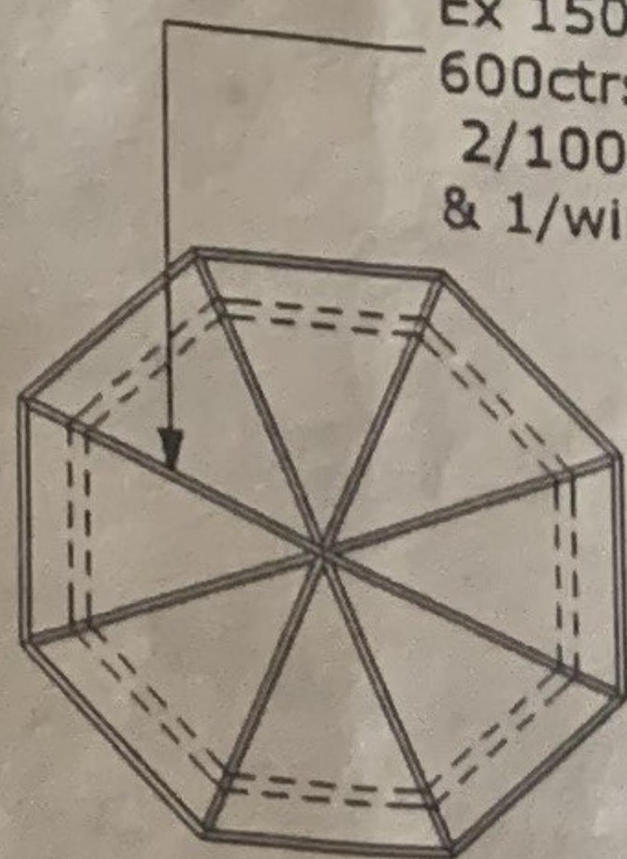
UPPER ROOF FRAMING PLAN
