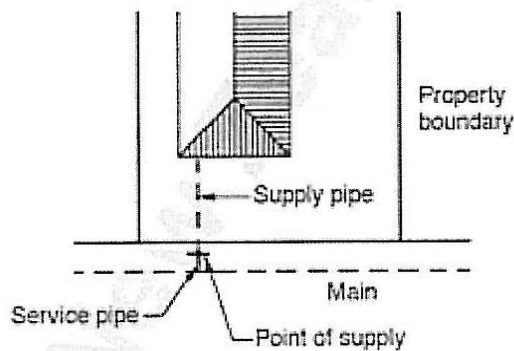
Type 2: Point of supply outside property boundary
