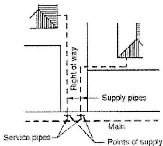
Type 2: Point of supply outside property boundary
